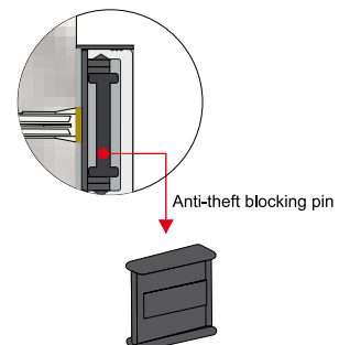
Cross-section JazZ side tracks
